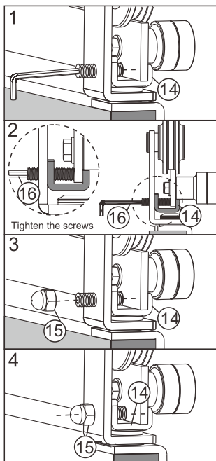
Installation procedure of fixed parts
