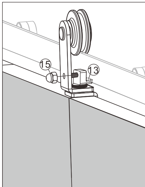
Sliding part structure
