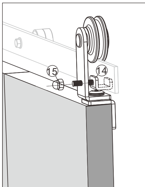
Fixed part structure
